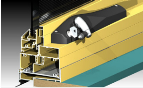
466 manual chainwinder comes standard with stainless chain, body can be coloured to match.
