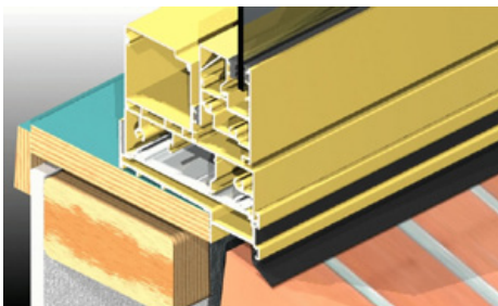
Custom sub-sill (flashing tray) standard on 466 windows.
