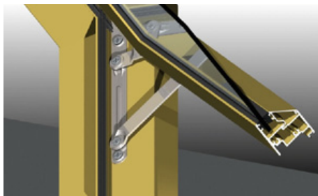
The 466 incorporates heavy duty friction or non-friction stays.
