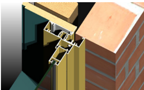
Nailing fin jamb standard on Series 461. Available in 30mm wide as shown or alternative 44mm.
