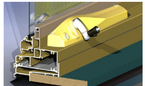
Manual chain winders are standard on Series 456 awning sashes.
