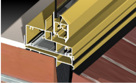
Series 456 windows come standard with integrated sub-sill.
