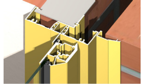
Standard 30mm nailing fin frame standard or alternative 44mm wide jamb.
